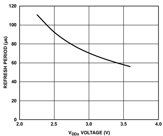
Figure 28. Typical Refresh Period vs. V_{DDx} Voltage
