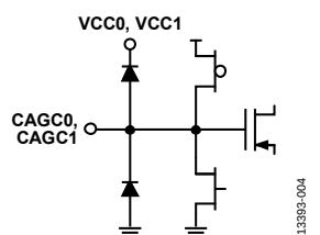
Figure 5. CAGCx Interface Schematic
