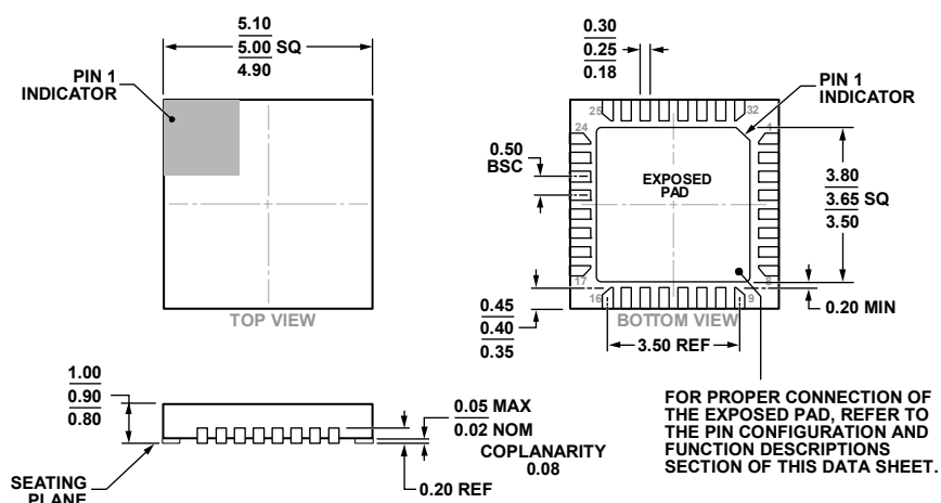
Figure 36.32-Lead Lead Frame Chip Scale Package [LFCSP] 5 mm × 5 mm Body and 0.90 mm Package Height (HCP-32-1)
