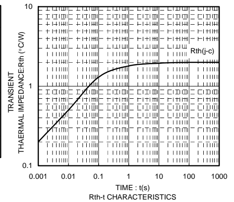
R_{th}(j-c) CHARACTERISTICS
