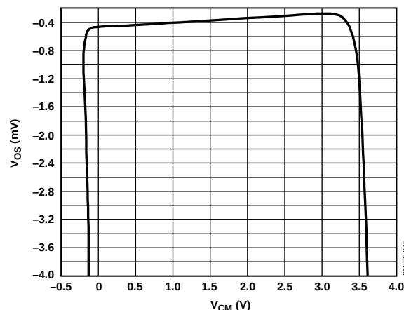
Figure 45. V_{os} vs. Common-Mode Voltage, V_s = 5 V
