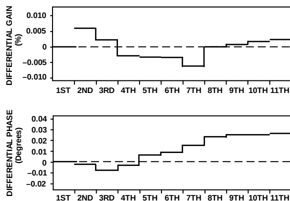
Figure 23. Differential Gain and Phase Error, G = 2 , NTSC Input Signal, R_L = 150 \Omega , V_S = 5 \text{ V}
