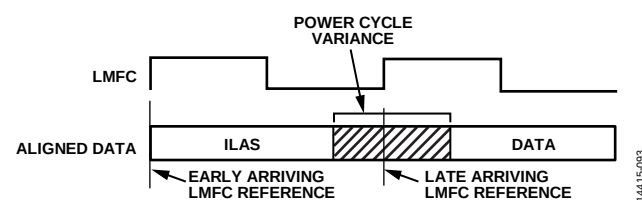
Figure 101. Link Delay &gt; LMFC Period Example
