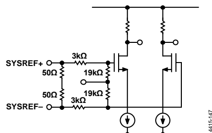
Figure 99. SYSREF± Input Circuit
