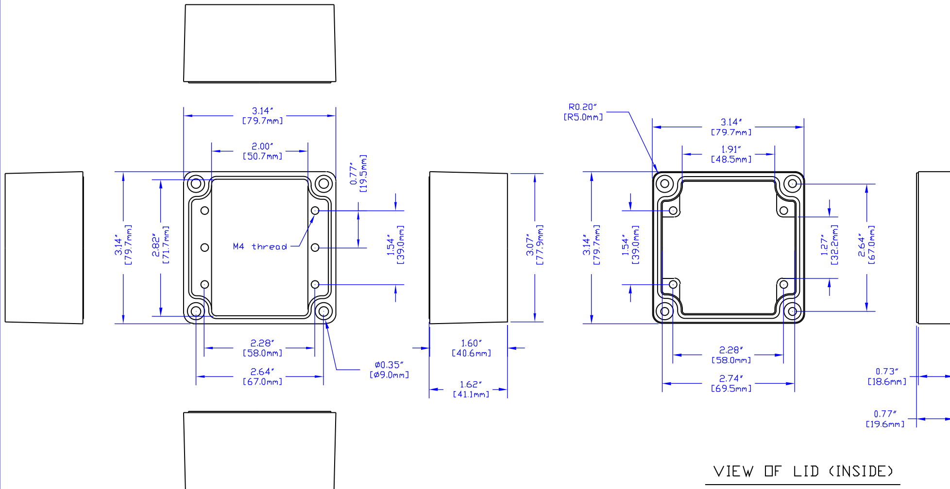
VIEW OF BOX (LID REMOVED)
