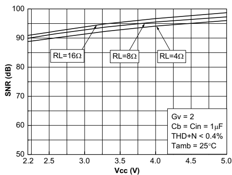
Figure 93. Signal-to-noise ratio vs power supply Gv=2
