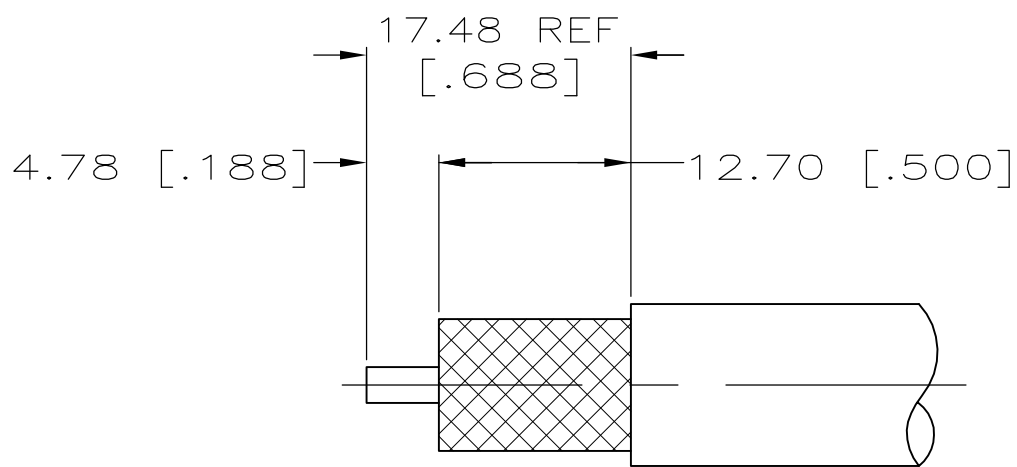
VIEW Y RECOMMENDED STRIP LENGTH SCALE 2:1
