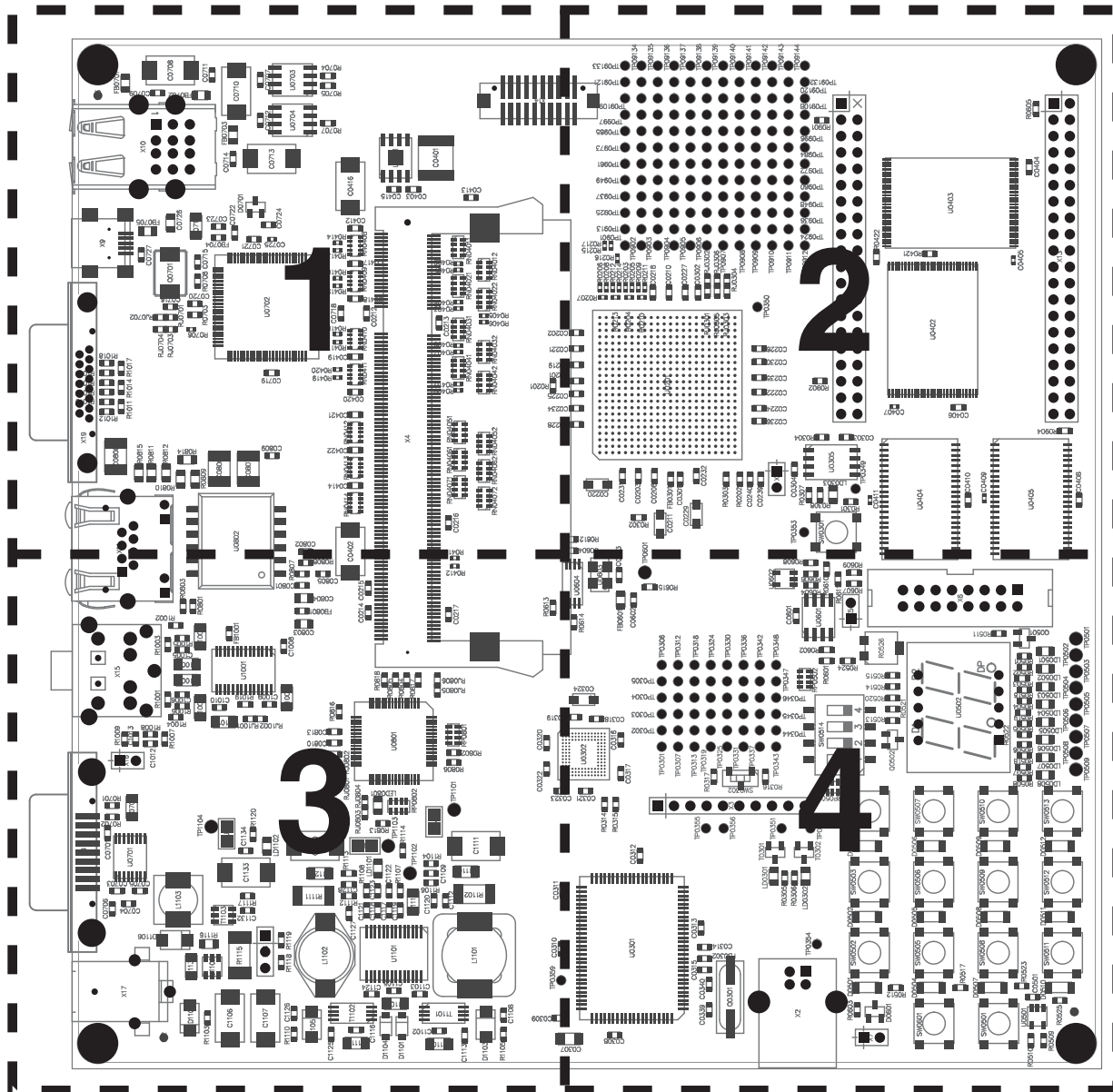
Figure 22. Assembly Diagram
