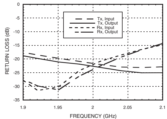
Return Loss with 2015 MHz Tuning
