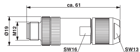
Plug, M12 x 1, straight, shielded
