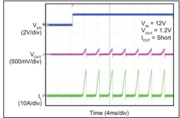
FIGURE 2-40: Enabled into Short.
