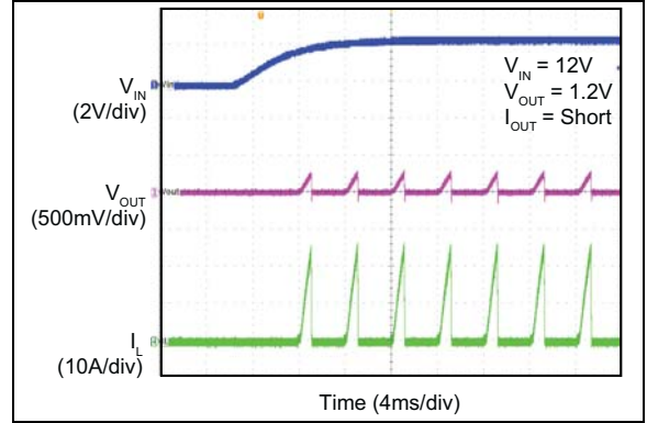
FIGURE 2-41: Power-Up into Short-Circuit.
