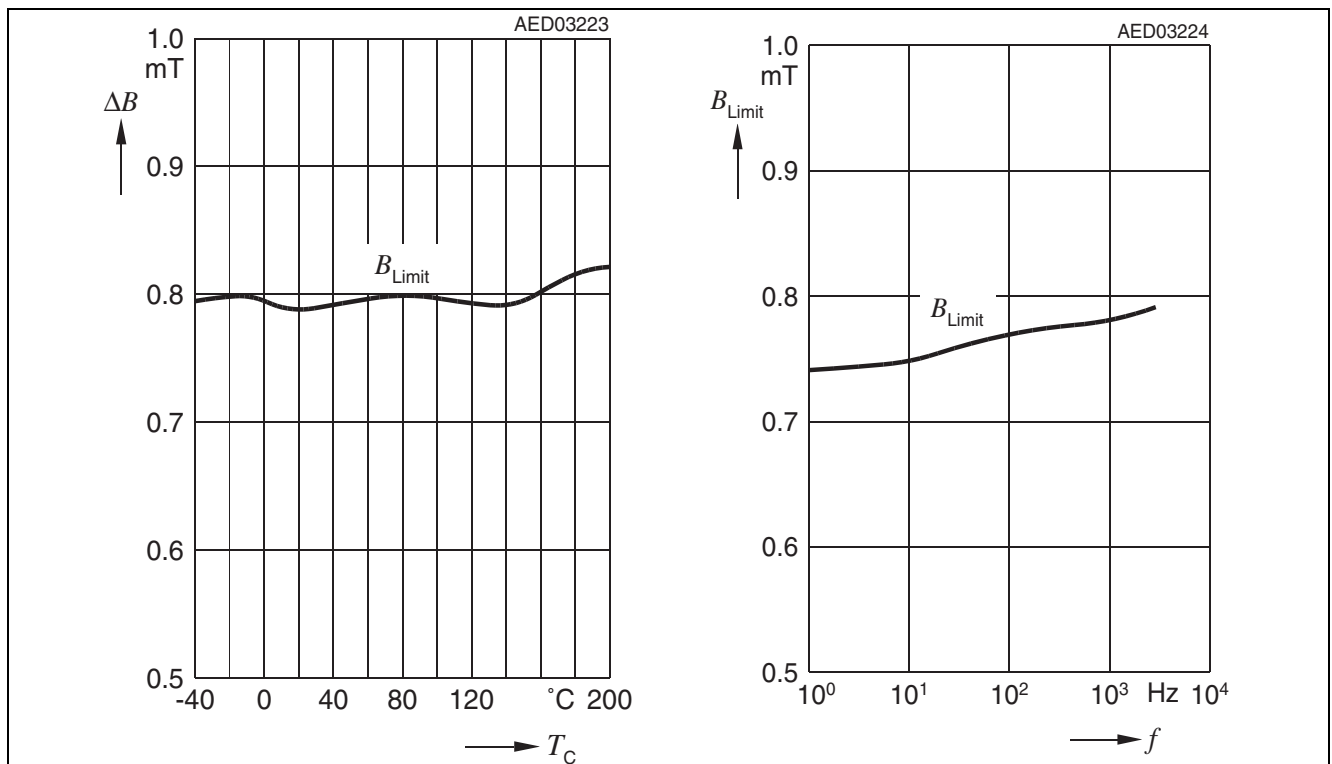
Figure 8 Magnetic Threshold \Delta B_{Limit} = f(T) at f = 1 kHz (left), Magnetic Threshold \Delta B_{Limit} = f(f) (right)
