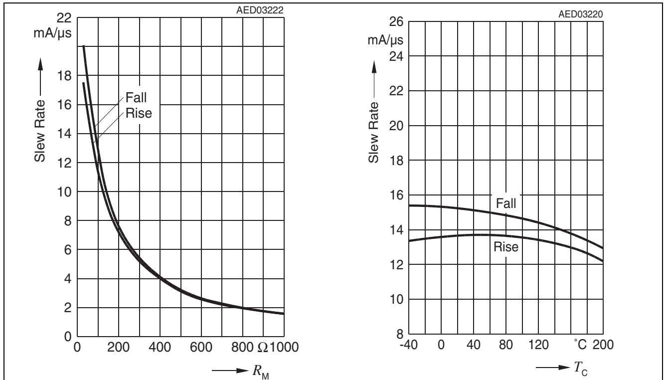
Figure 7 Slew Rate with C = 1.8 nF = f(R_M) (left), Slew Rate with C = 1.8 nF, R_M = 75 Ω (right)
