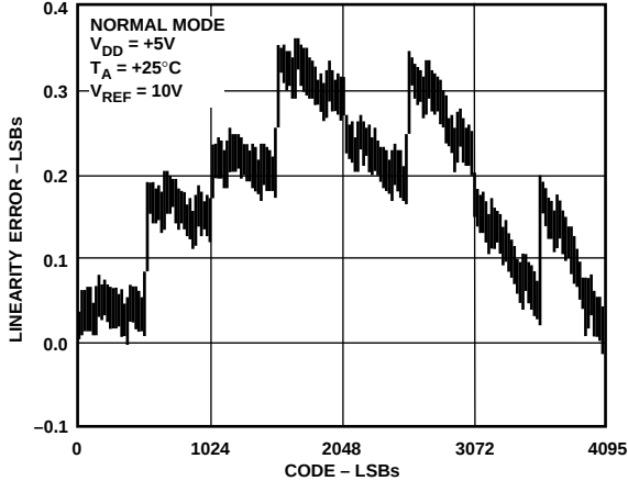
Figure 14. All Codes Linearity Plot (Normal Mode)
