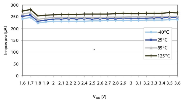
Figure 8. I_{DD(WAIT)} vs. V_{DD} , f_{CPU} = 2 \text{ MHz}
