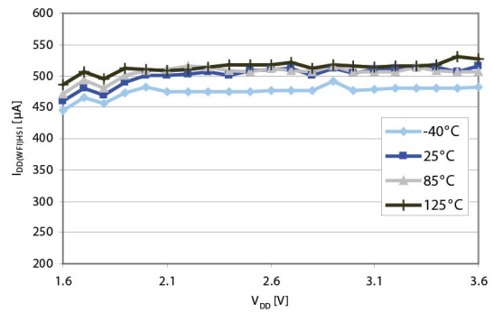
Figure 9. I_{DD(WAIT)} vs. V_{DD} , f_{CPU} = 16 \text{ MHz}
