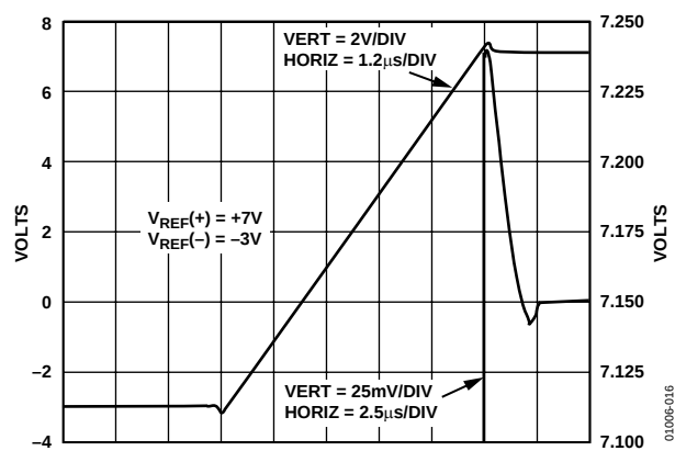
Figure 16. Settling Time(+)
