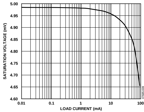
Figure 39. Output Saturation Voltage vs. Load Current
