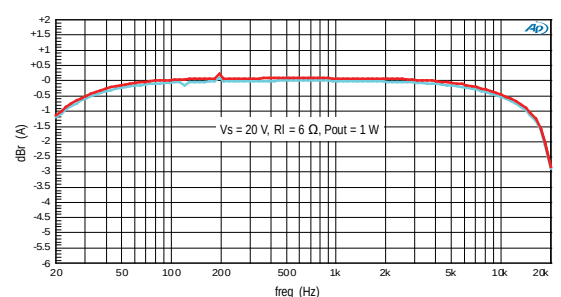
Figure 13: Frequency response
