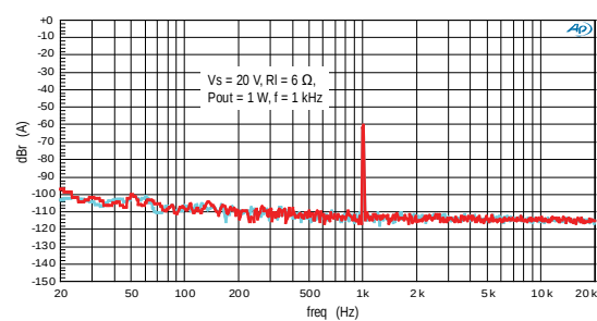
Figure 15: FFT (-60 dB)
