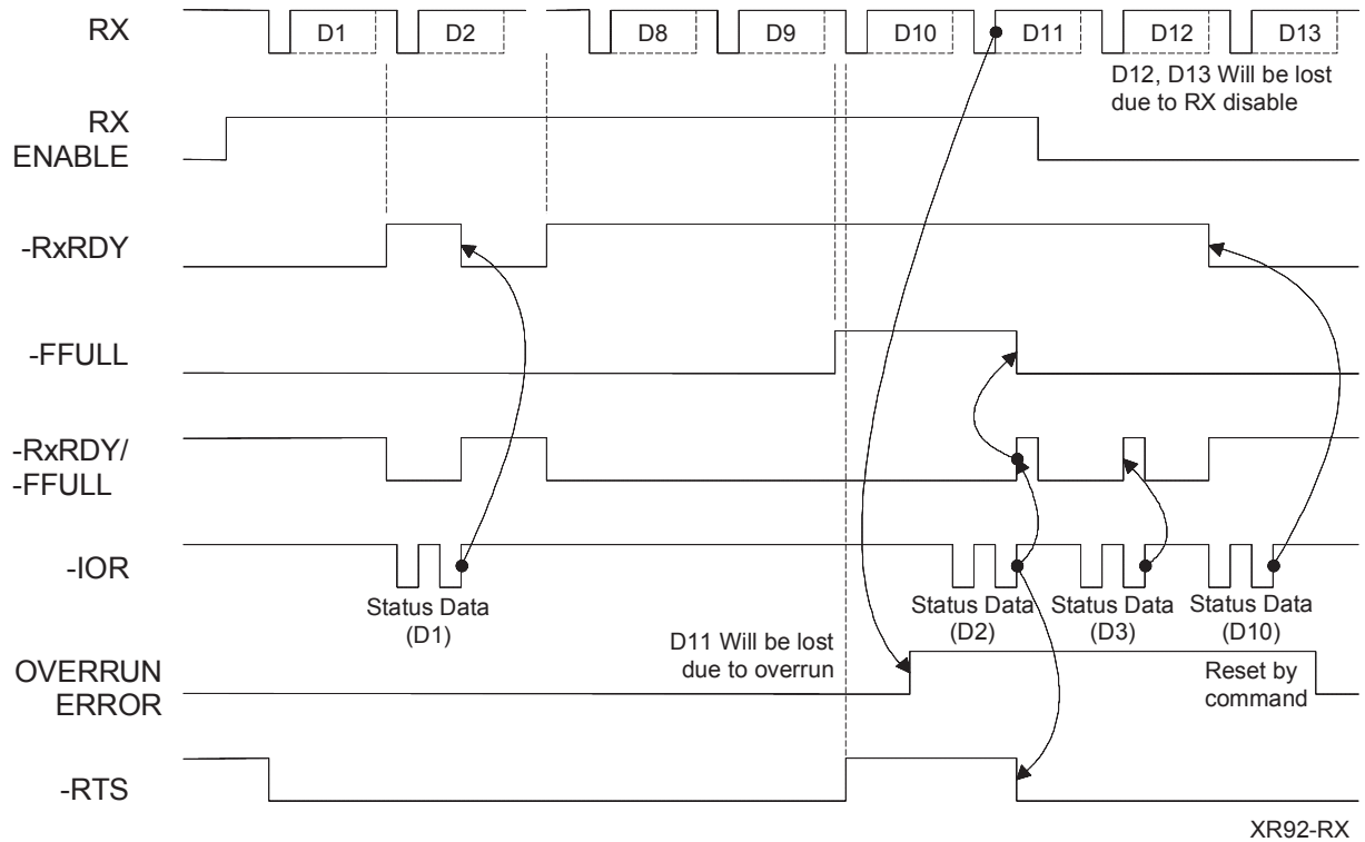
Figure 6: Receive Timing
