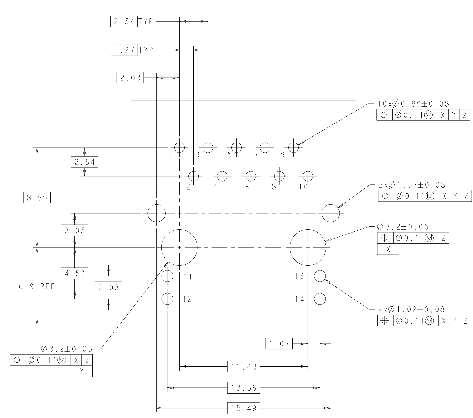
SUGGESTED CUSTOMER BOARD LAYOUT (COMPONENT SIDE)
