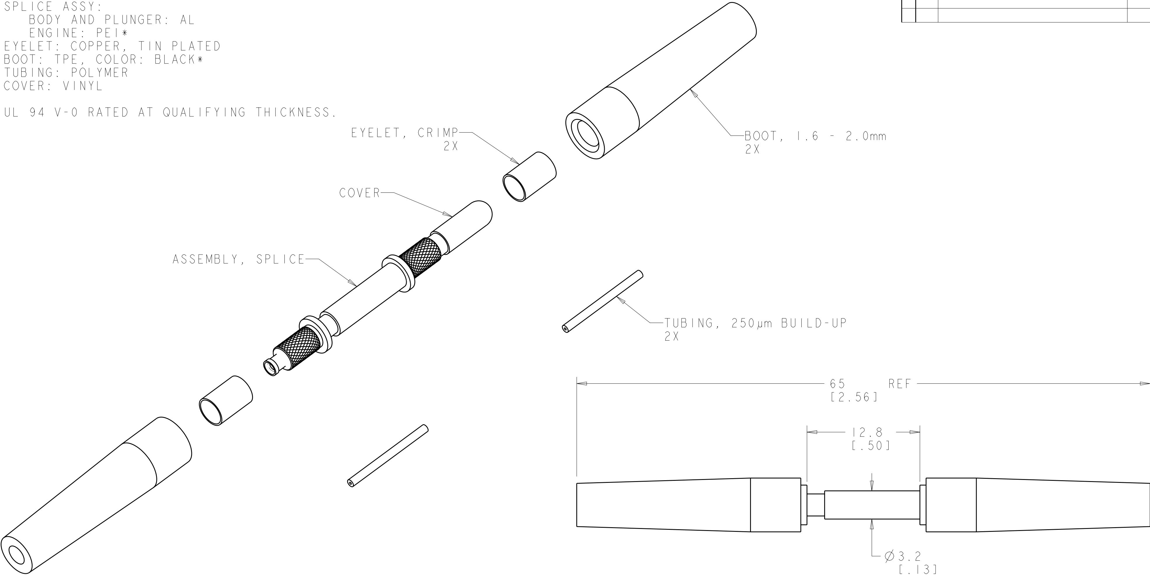
CLOSED ASSEMBLY
