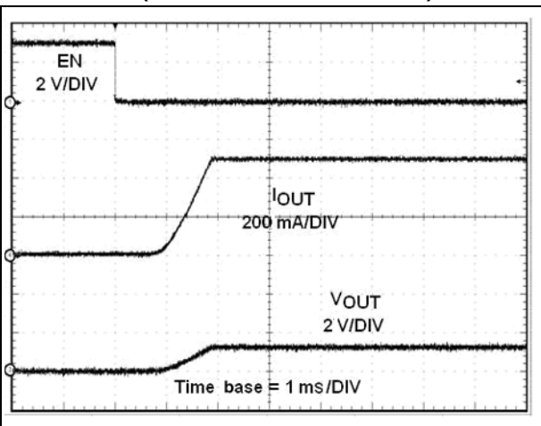
Figure 14. OC protection at V OUT = 3.0 V (STMPS2141/2151 - detail)
