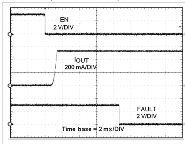
Figure 13. OC protection at V OUT = 3.0 V (STMPS2141/2151)
