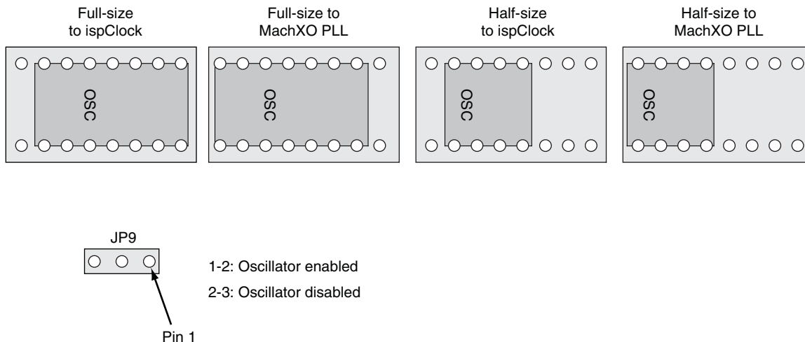
Figure 6. Oscillator Positions
