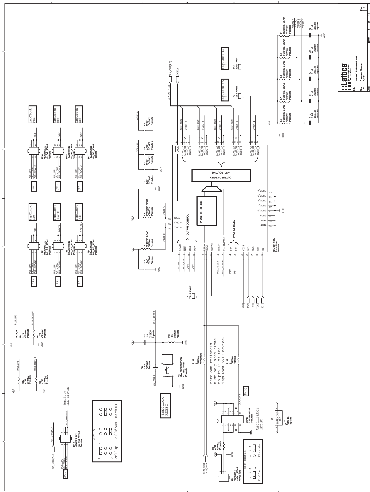
Figure 12. ispClock5610 Connections
