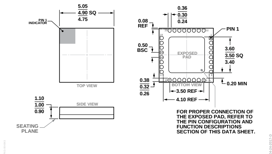
Figure 18. 32-Terminal Ceramic Leadless Chip Carrier [LCC] (E-32-1) Dimensions shown in millimeters
