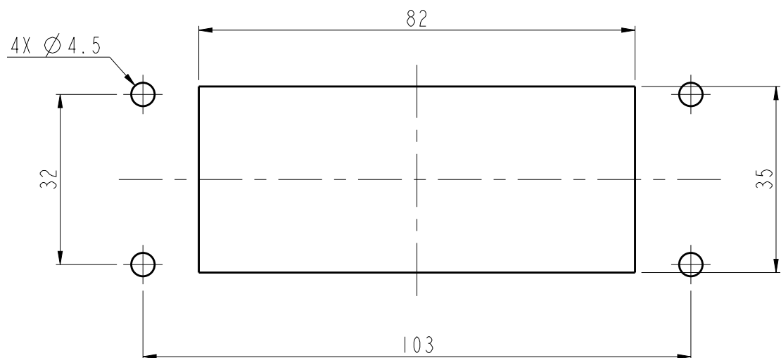
RECOMMENDED PANEL CUT OUT DIMENSIONS 推荐面板开孔尺寸
