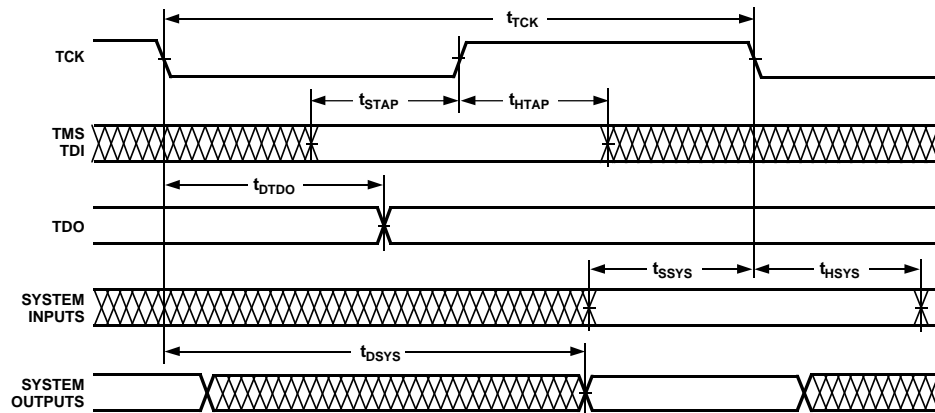
Figure 25. IEEE 11499.1 JTAG Test Access Port
