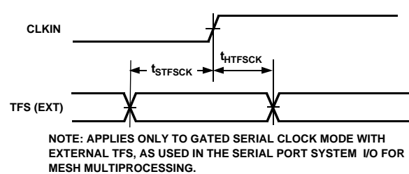
Figure 24. Serial Ports
