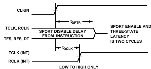
Figure 24. Serial Ports
