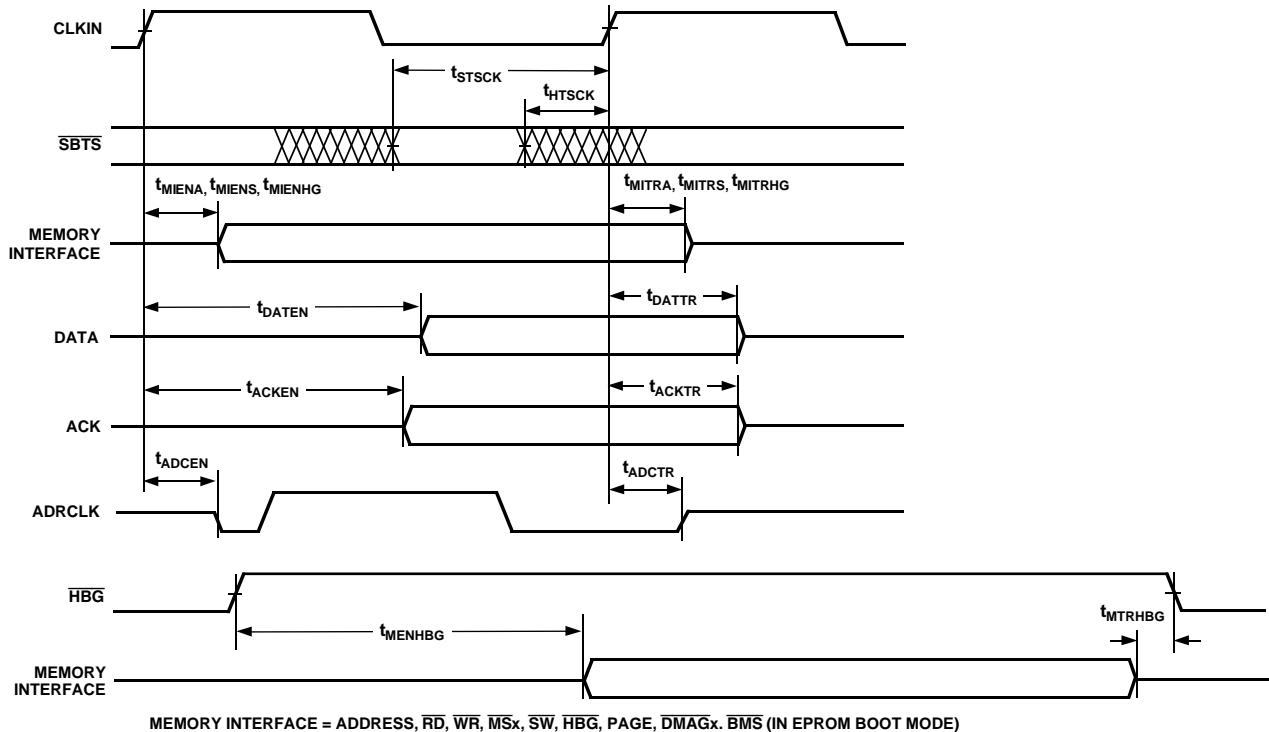
Figure 20. Three-State Timing
