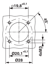
Installation dimensions
