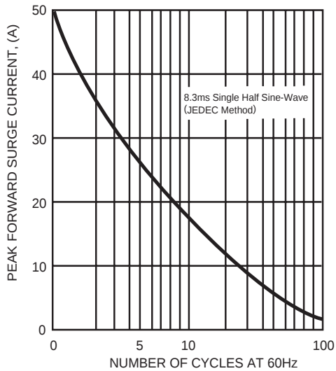
FIG. 1 - MAXIMUM NON-REPETITIVE SURGE CURRENT
