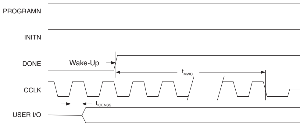
Figure 3-27. Wake-Up Timing
