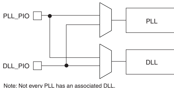
Figure 2-7. Sharing of PIO Pins by PLLs and DLLs in LA-LatticeECP3 Devices
