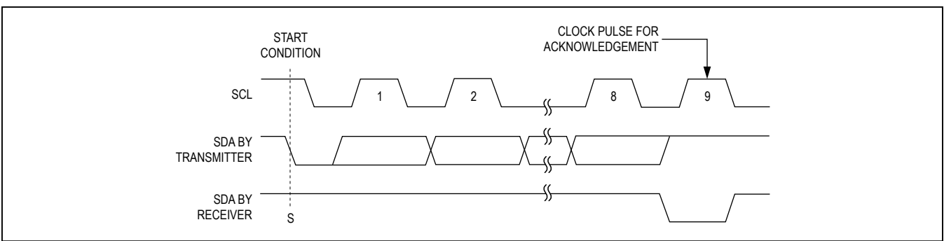
Figure 9. Acknowledge
