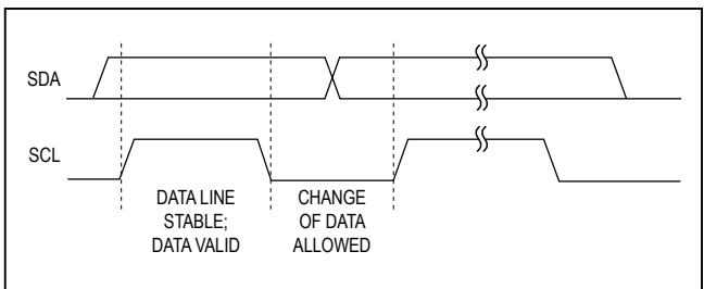
Figure 8. Bit Transfer
