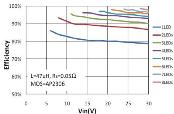
Efficiency vs. No. of LEDs
