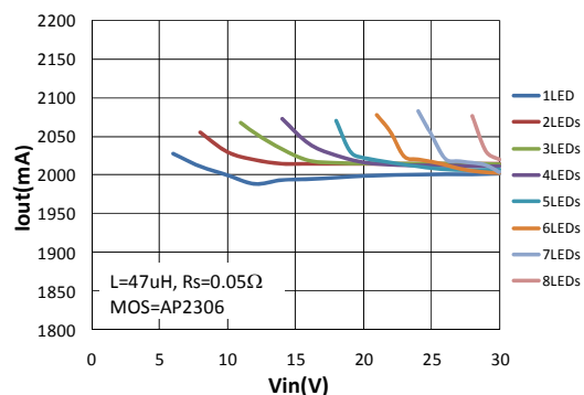
Output current variation with Supply Voltage
