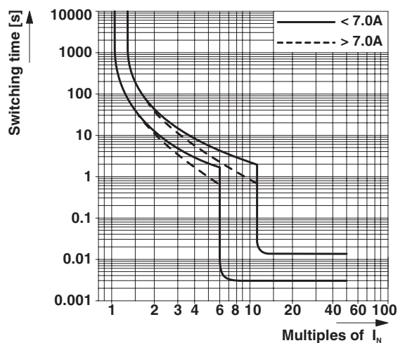
Figure 1 AC and DC tripping characteristics
