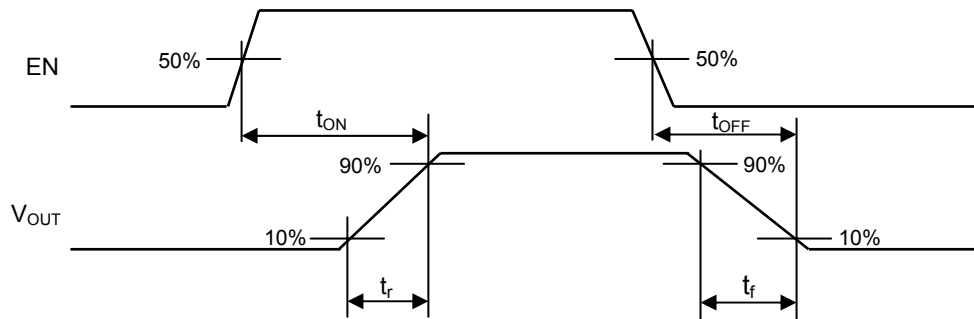
Figure 5. Timing Diagram
