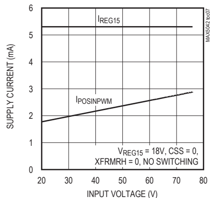
POSINPWM INPUT CURRENT, REG15 INPUT CURRENT vs. INPUT VOLTAGE
