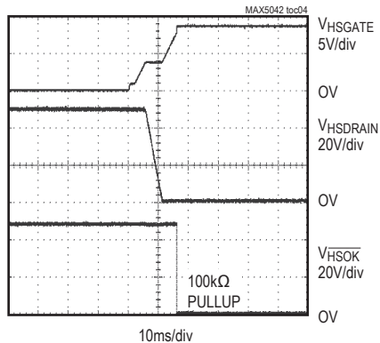
HOT-SWAP STARTUP WAVEFORM
