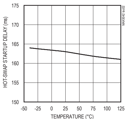
HOT-SWAP STARTUP DELAY vs. TEMPERATURE
