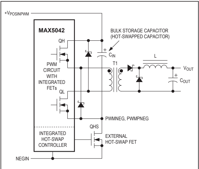
Figure 1. Simplified Diagram of a MAX5042-Based Isolated Power Supply
