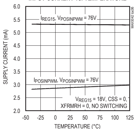
POSINPWM INPUT CURRENT, REG15 INPUT CURRENT vs. TEMPERATURE
