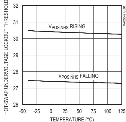
HOT-SWAP UNDERVOLTAGE LOCKOUT THRESHOLD vs. TEMPERATURE
