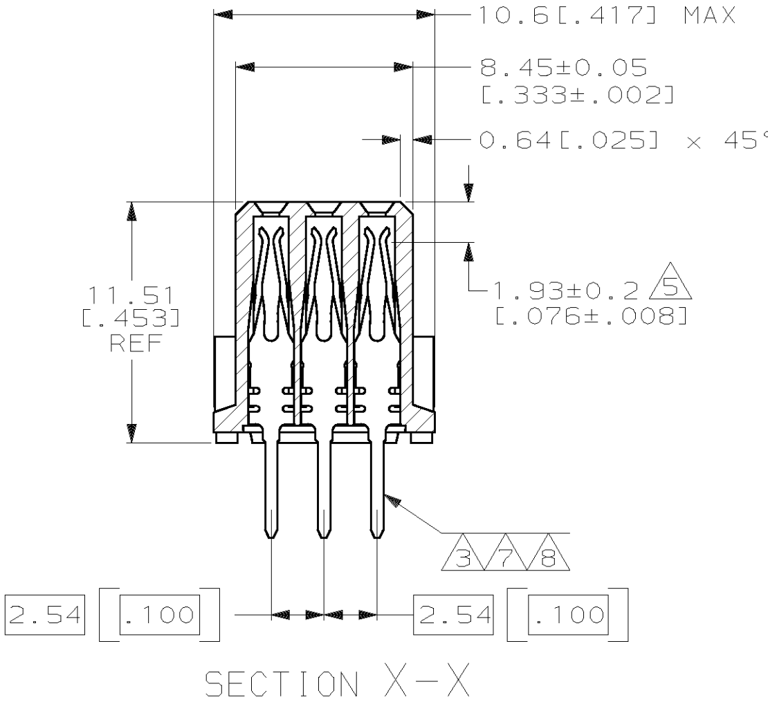
SECTION X-X
