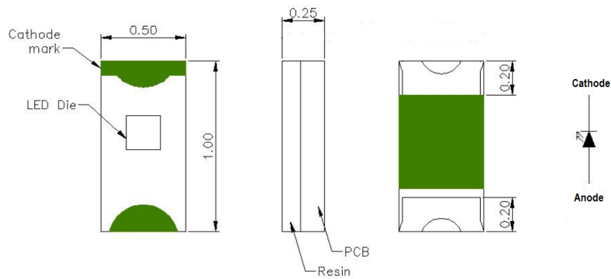
Figure 1: Package Dimensions
