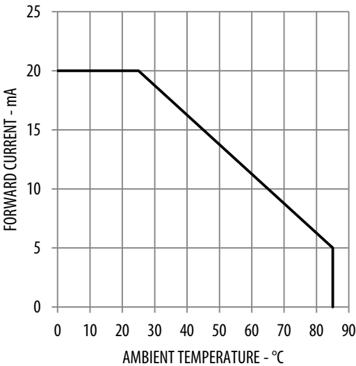
Figure 10: Derating Curve
