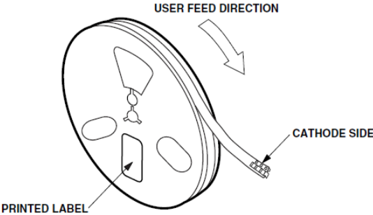
Figure 12: Reel Orientation
