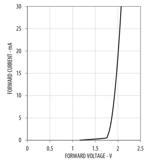
Figure 4: Forward Current vs. Forward Voltage
