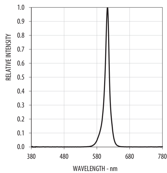
Figure 2: Spectrum
