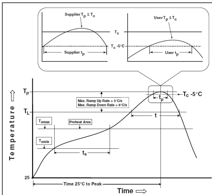
Figure 35 Classification Profile
