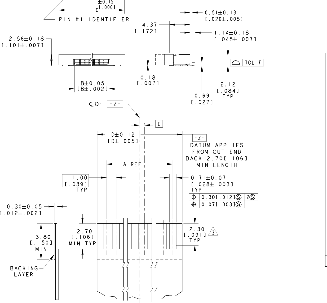
RECOMMENDED FPC LAYOUT SCALE 8:1
