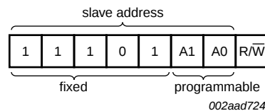
Fig 8. PCA9539; PCA9539R device address
