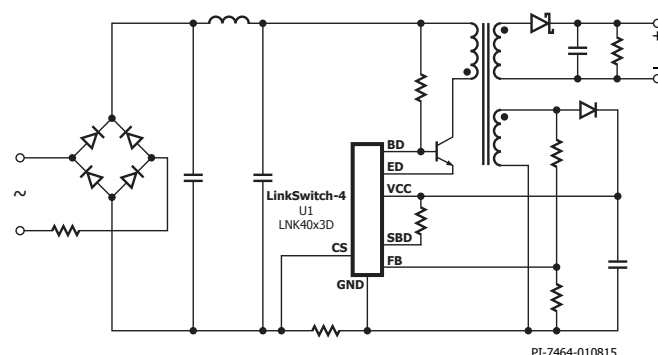
Figure 2. Typical Application (SO-8) (D).
