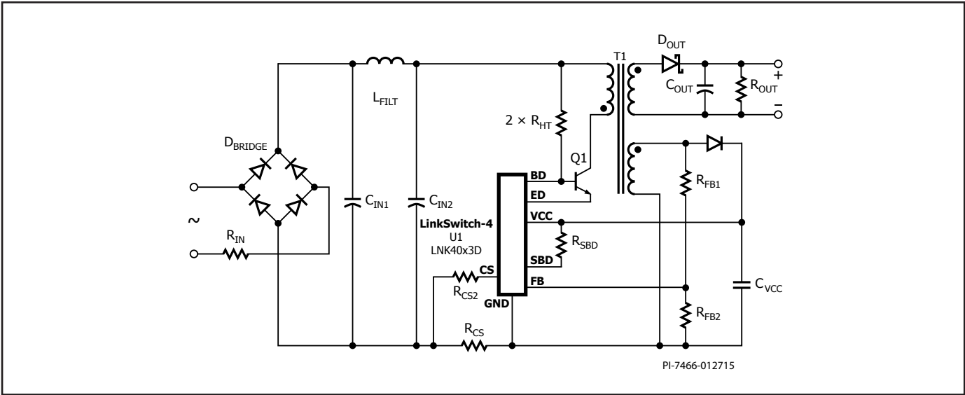
Figure 10. Typical Universal Input, 10 W Charger.
