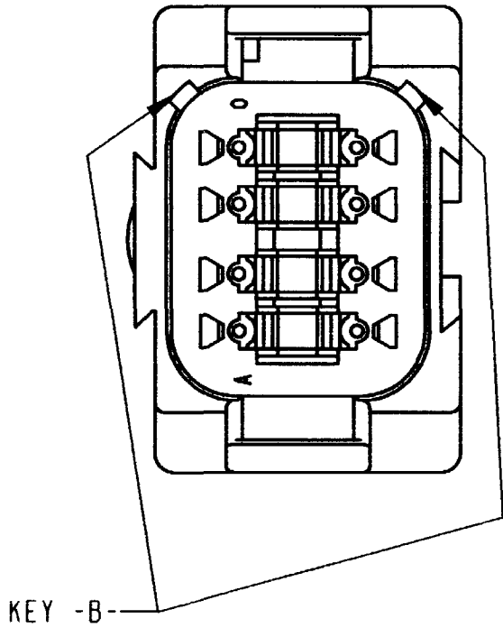
PART NO. DT04-08PB-CE01 KEY ARRANGMENT -B- COLOR: BLACK
