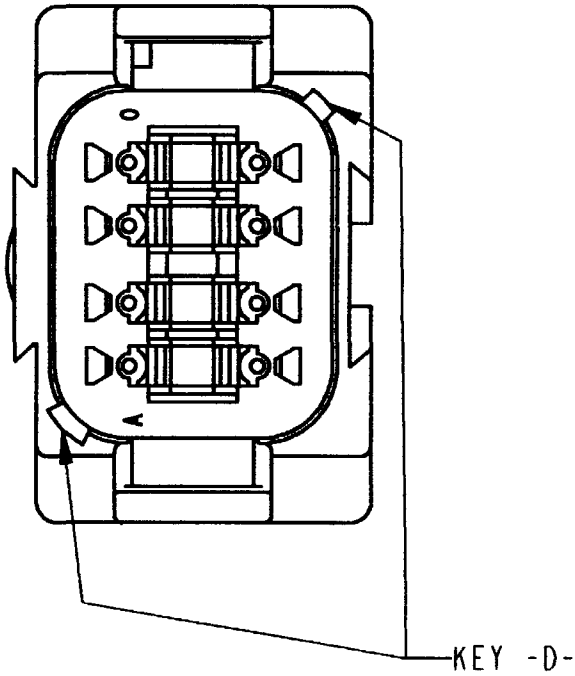
PART NO. DT04-08PD-CE01 KEY ARRANGMENT -D- COLOR: BROWN
