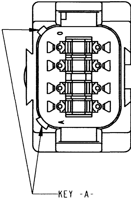
PART NO. DT04-08PA-CE01 KEY ARRANGMENT -A- COLOR: GRAY
