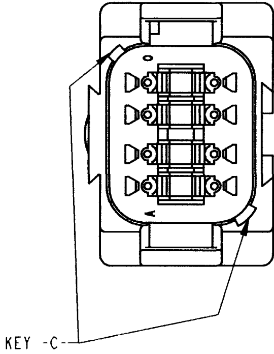
PART NO. DT04-08PC-CE01 KEY ARRANGMENT -C- COLOR: GREEN
