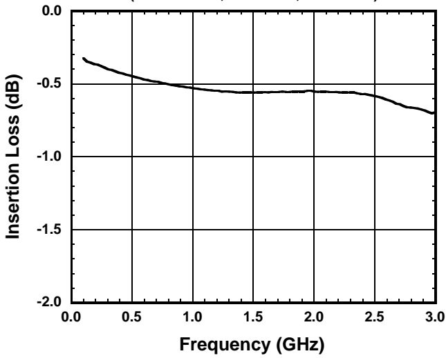
RX-ANT1 Insertion Loss vs. Frequency
