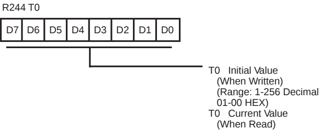
Figure 49. Counter/Timer 0 Register F4H; Read/Write
