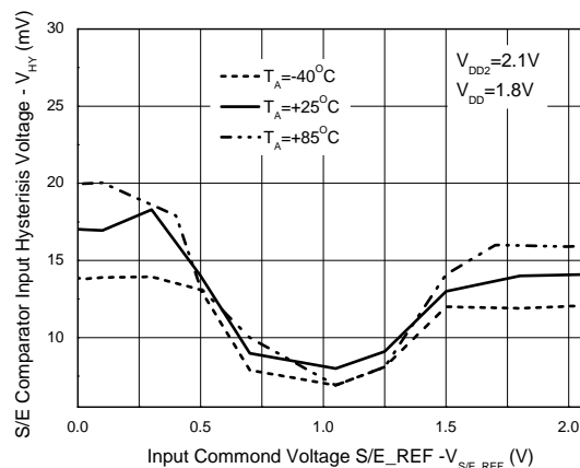
S/E Comparator Input Internal Hysteresis Voltage Characteristics
