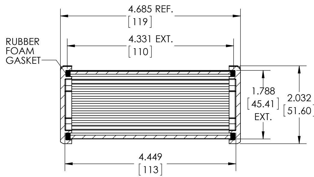
SECTION A-A DIMENSIONS MAY VARY DEPENDING ON THE COMPRESSION OF THE GASKETS
