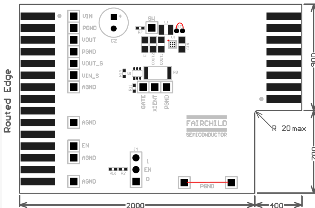
Figure 3. Top-Side Silk Screen
